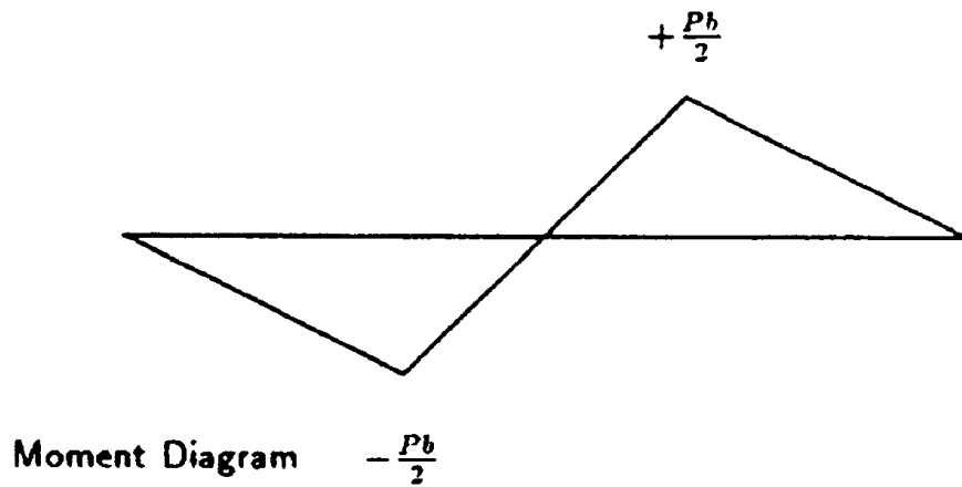
Shear Diagram
