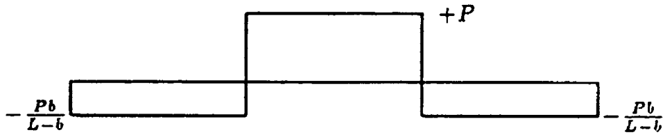
Force Diagram
